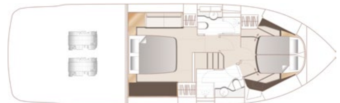
LOWER DECK
